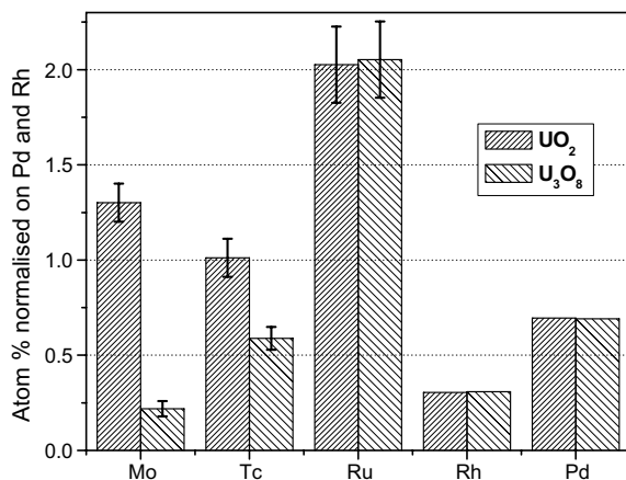
Fig. 6. EDX analysis of the metallic precipitates in irradiated \text{UO}_2 and \text{U}_3\text{O}_{8-x} annealed at 1900 K: average composition histograms. The values were normalised to Rh + Pd.
